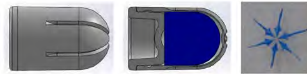
Current 9mm FX ® PROJECTILE
