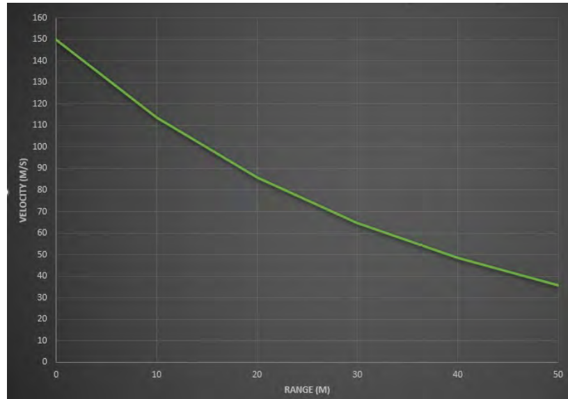
Decrease in velocity over distance
